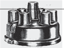
AL 99 Suppression Cap - 8 Cyl. equipped with AL 119 10,000 ohm. Suppression Brush (3-2) (IAR-1003) used with AL 65 Rotor
